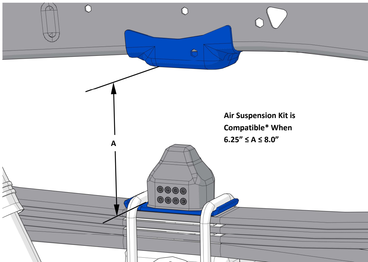
Figure 1. Diagram of GM Colorado/Canyon Rear Suspension
