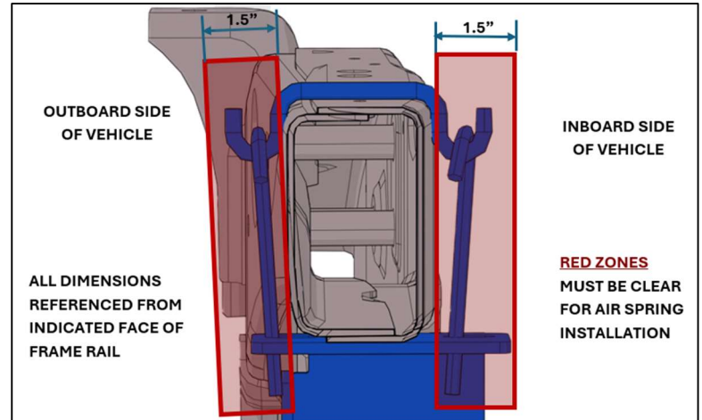
Figure 1. Clearance Requirements, Part 1
