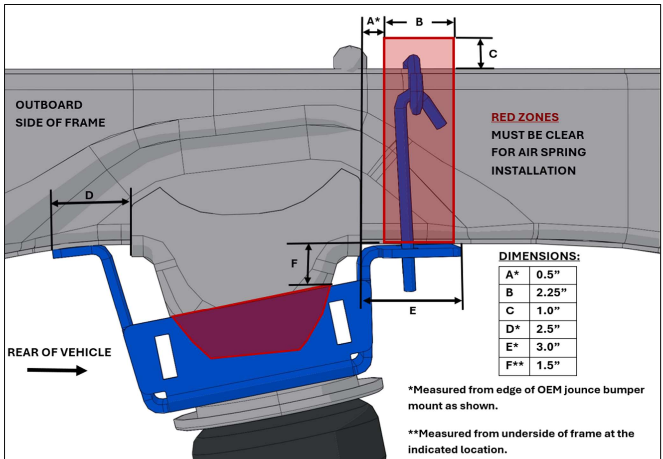
Figure 2. Clearance Requirements, Part 2
