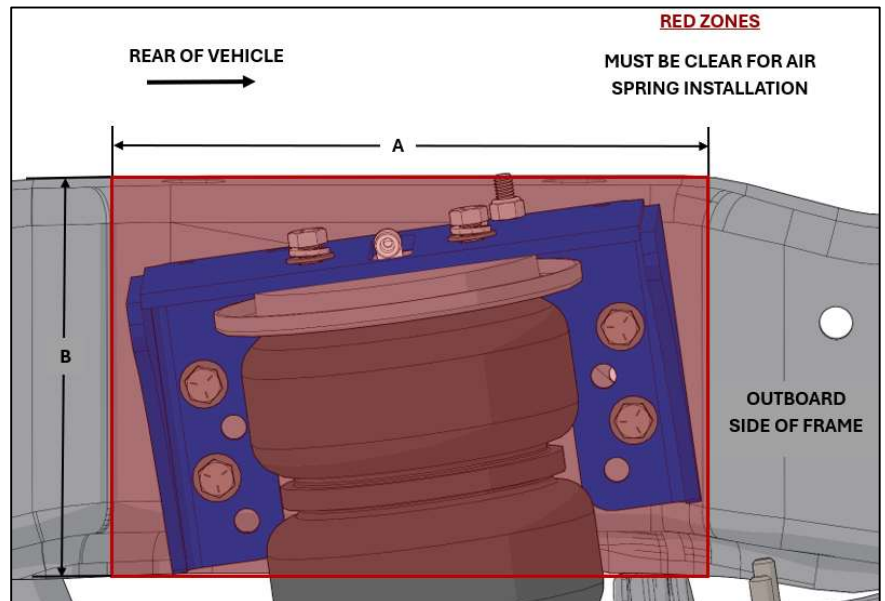
Figure 1. Clearance Requirements, Part 1
