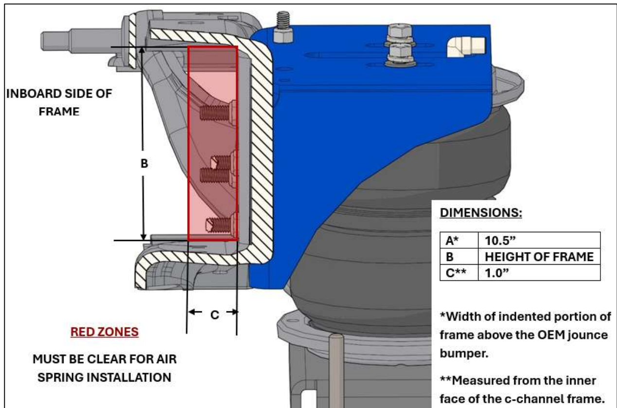
Figure 2. Clearance Requirements, Part 2
