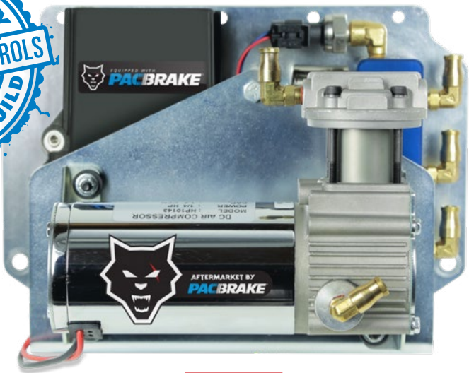
Tankless Onboard Air Kit
